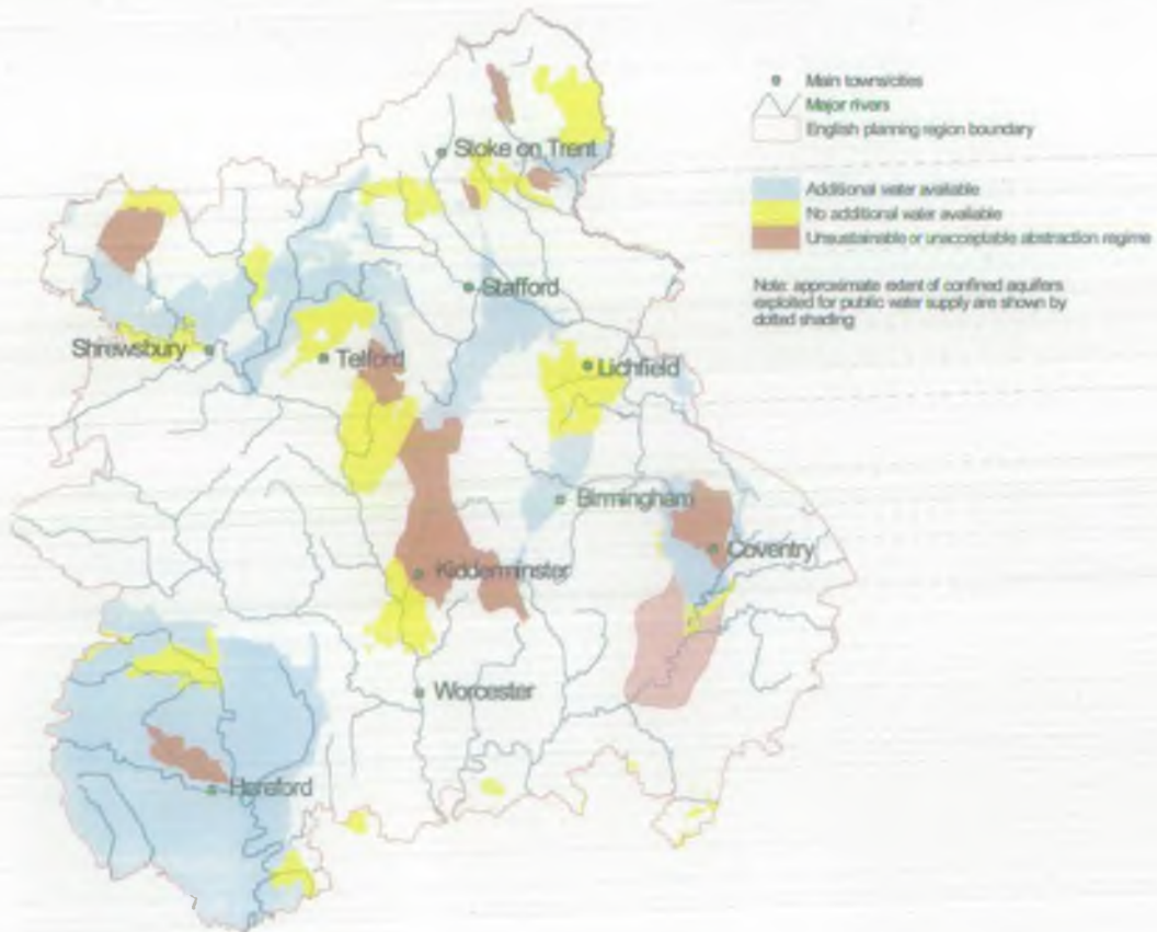
Figure 4 Current indicative availability of water resources: groundwater
