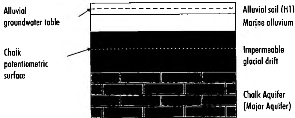
FIGURE 5.1 Diagrammatic cross section of the possible misrepresentation of the groundwater vulnerability of some confined aquifers.
