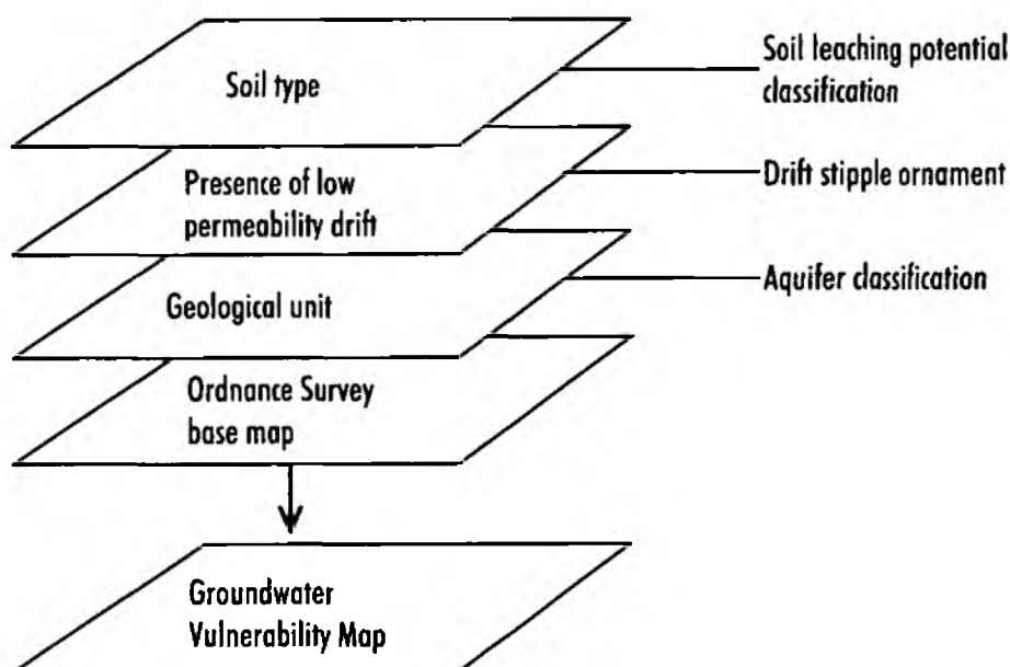
FIGURE 1.1 Overview of information layers used to compile a Groundwater Vulnerability Map
